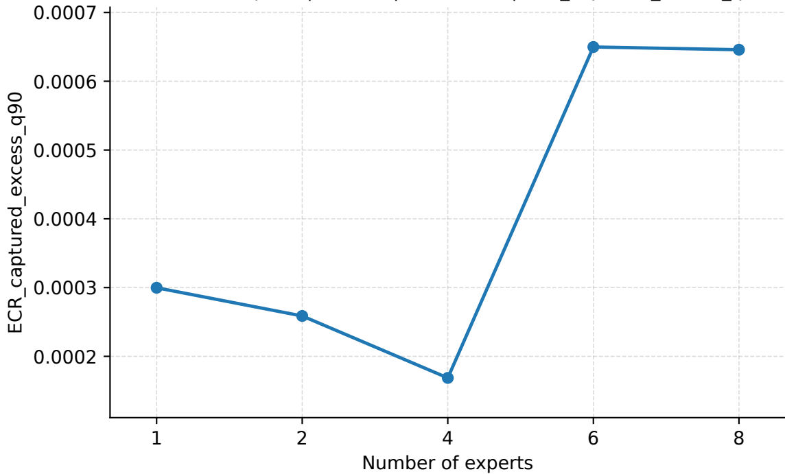
Number of Experts | Abilene | PredLen=5 | ECR_captured_excess_q90
