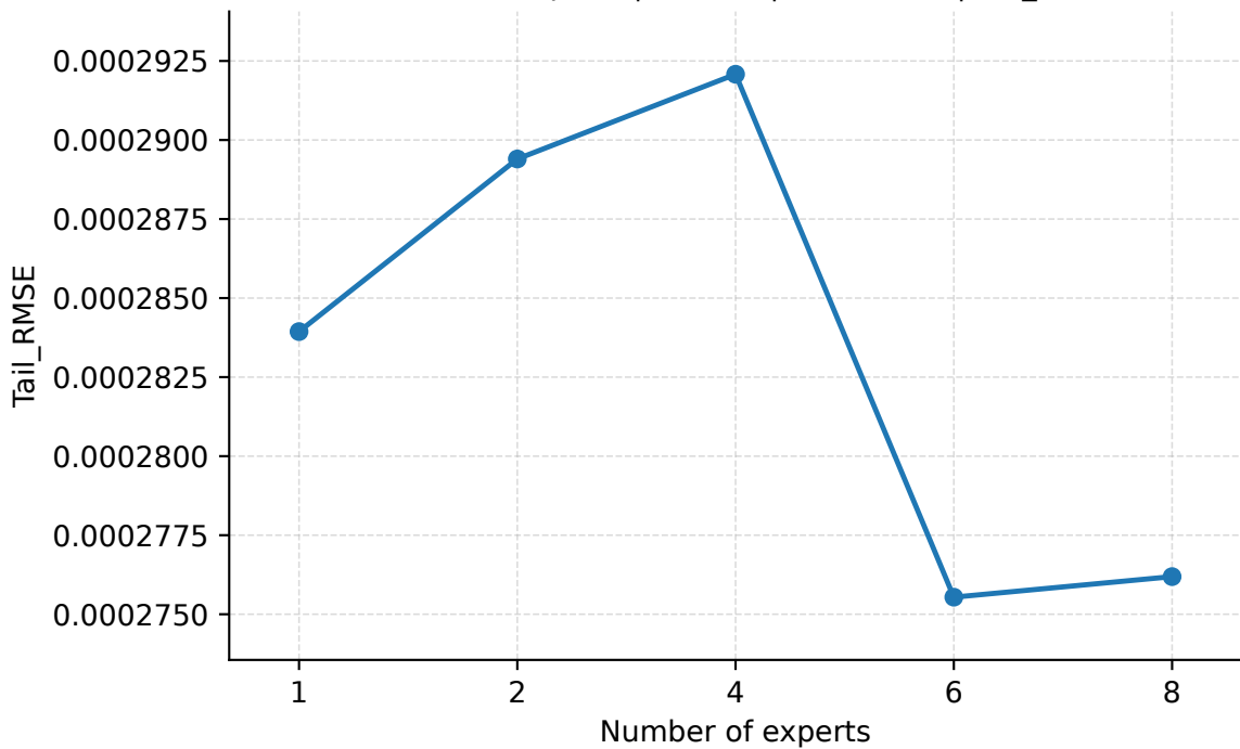
Number of Experts | Abilene | PredLen=5 | Tail_RMSE
