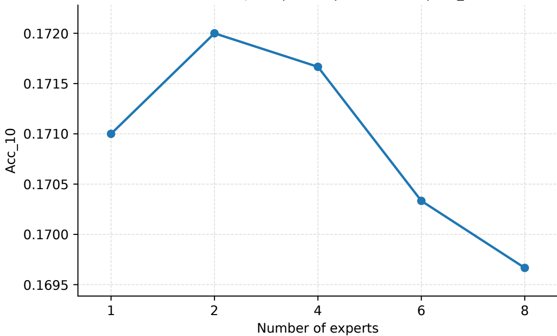
Number of Experts | Geant | PredLen=10 | Acc_10
