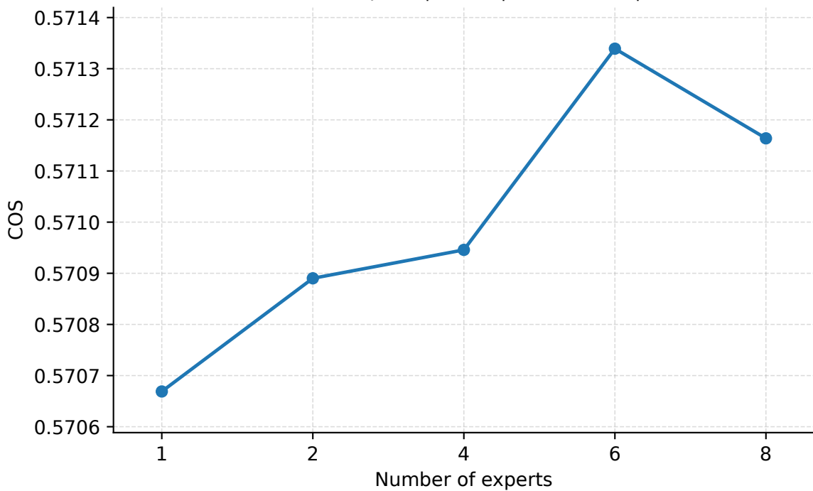
Number of Experts | Geant | PredLen=10 | COS
