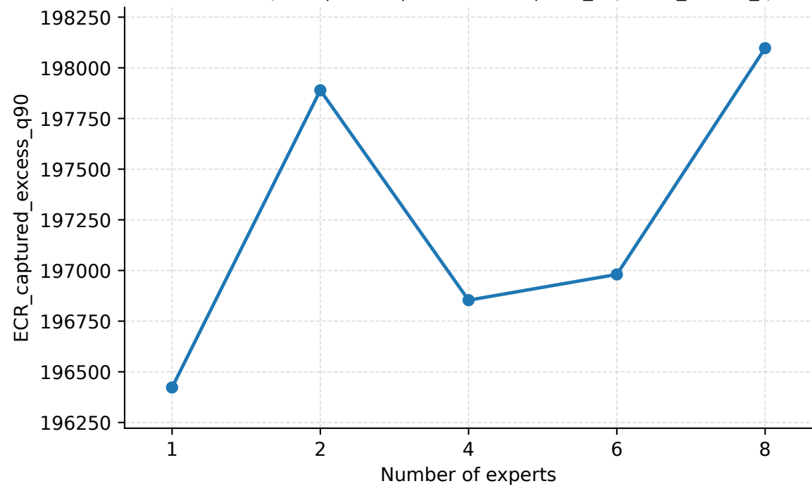
Number of Experts | Geant | PredLen=10 | ECR_captured_excess_q90
