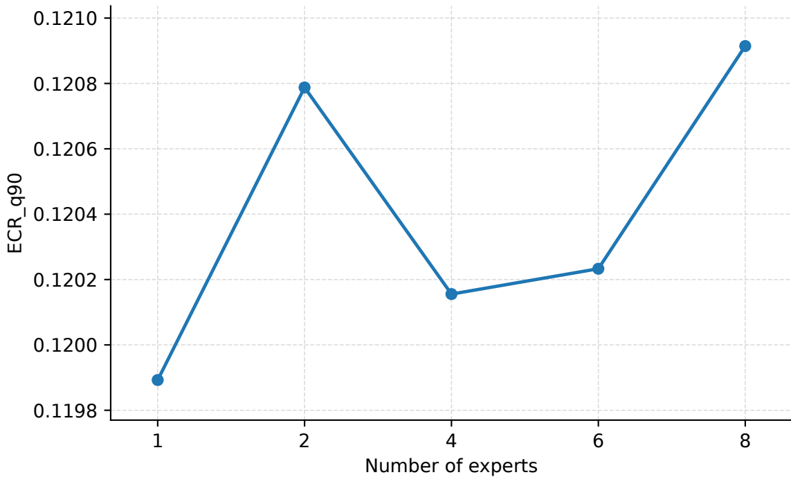
Number of Experts | Geant | PredLen=10 | ECR_q90
