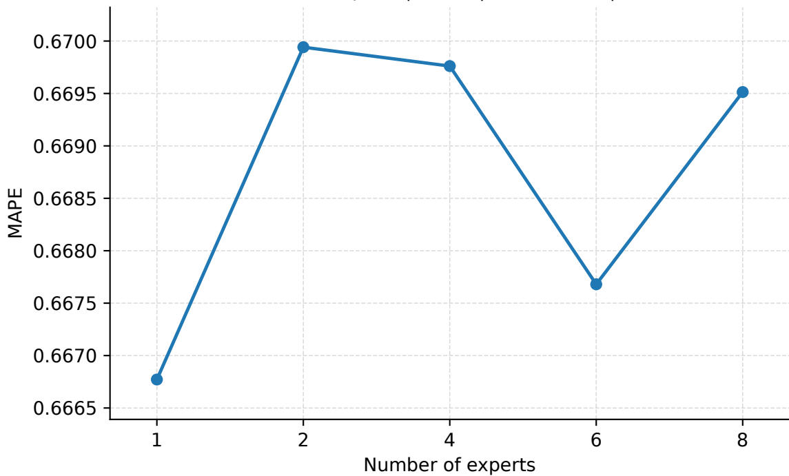
Number of Experts | Geant | PredLen=10 | MAPE
