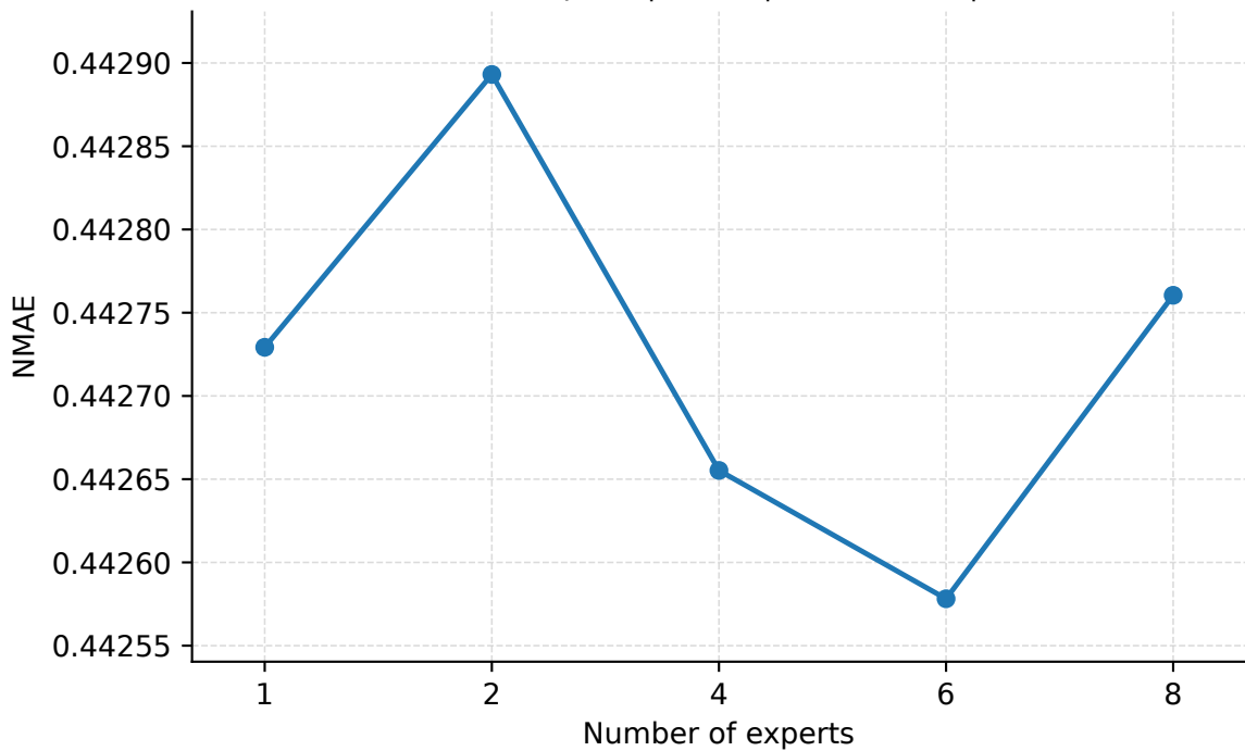
Number of Experts | Geant | PredLen=10 | NMAE
