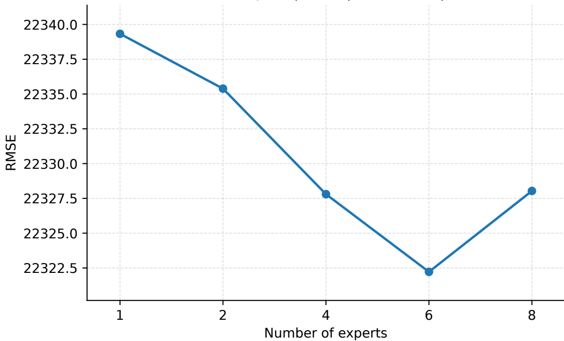
Number of Experts | Geant | PredLen=10 | RMSE
