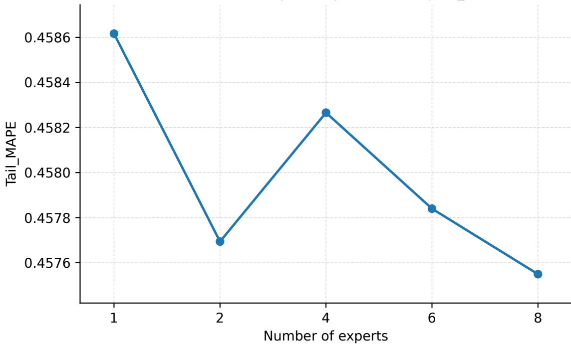
Number of Experts | Geant | PredLen=10 | Tail_MAPE
