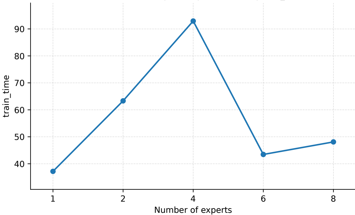
Number of Experts | Geant | PredLen=10 | train_time
