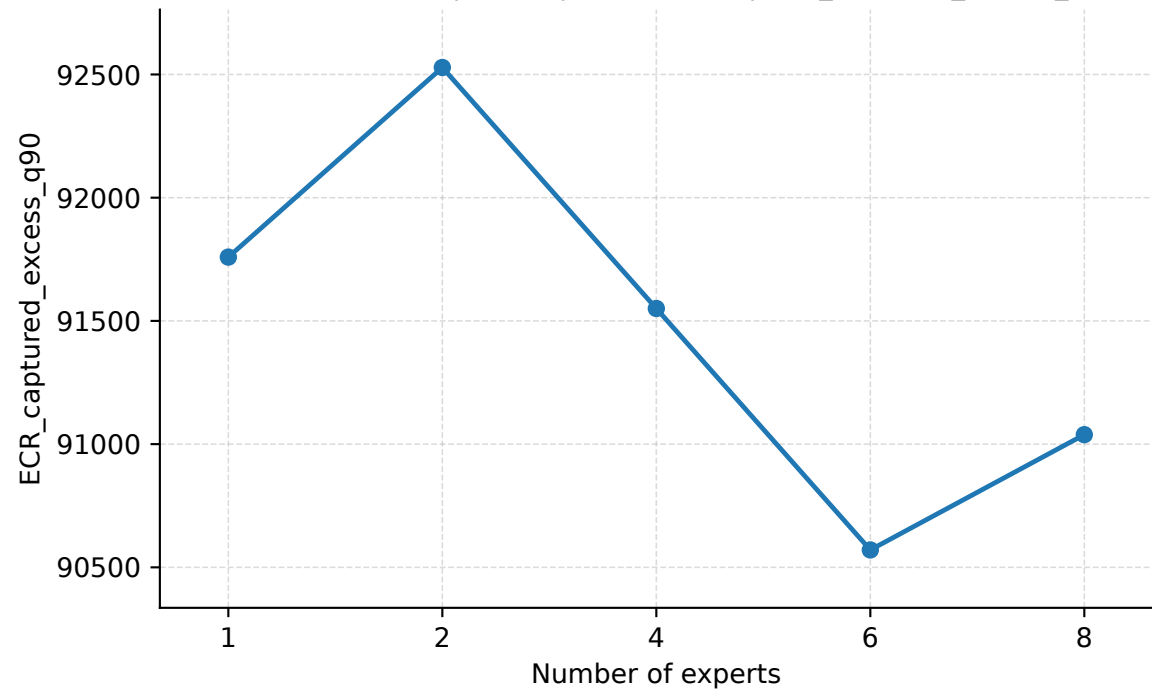
Number of Experts | Geant | PredLen=15 | ECR_captured_excess_q90
