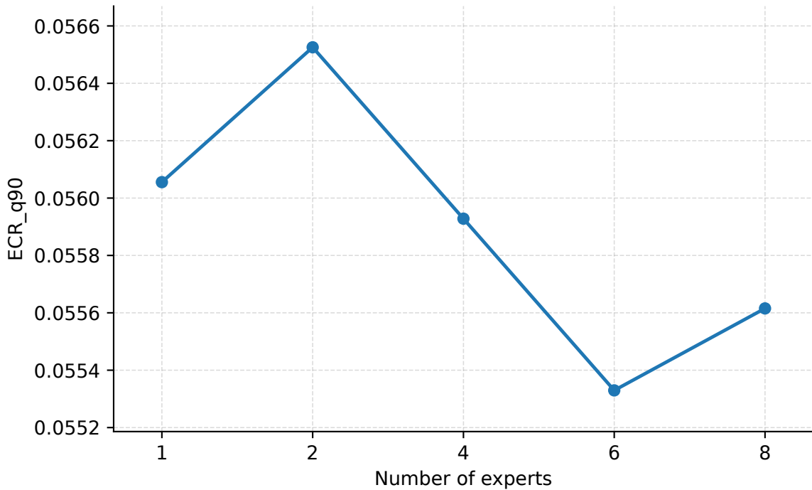
Number of Experts | Geant | PredLen=15 | ECR_q90
