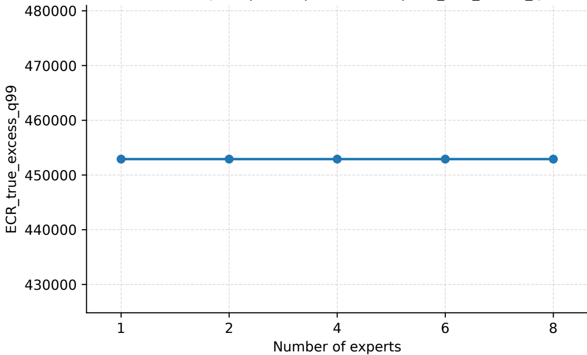
Number of Experts | Geant | PredLen=15 | ECR_true_excess_q99
