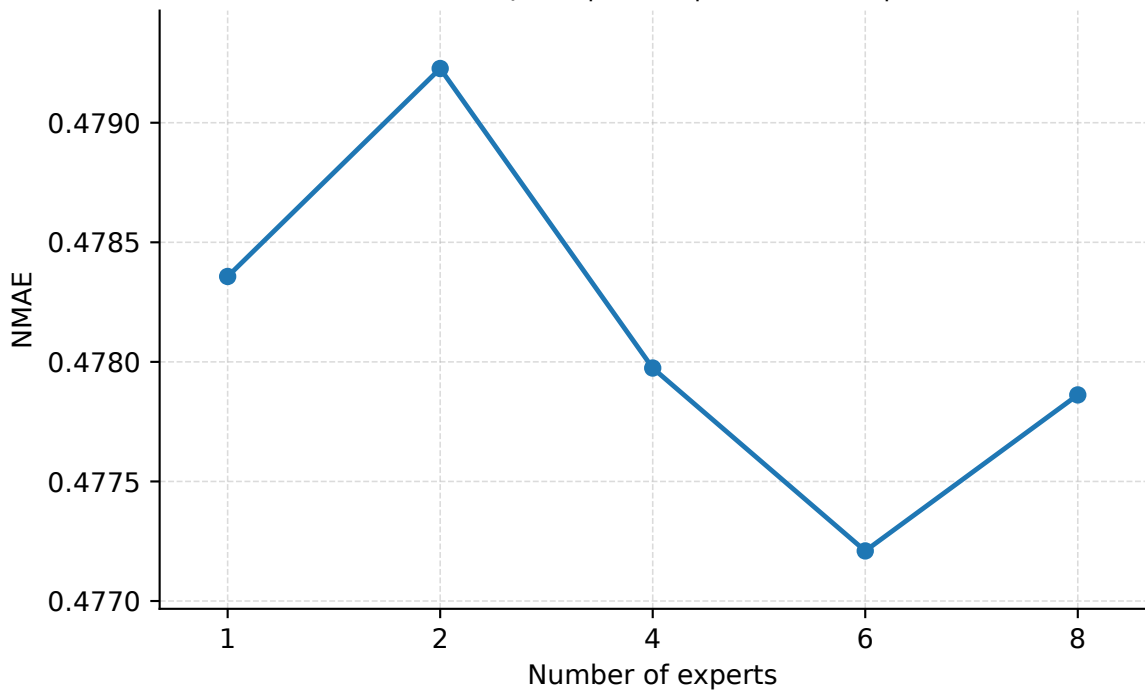
Number of Experts | Geant | PredLen=15 | NMAE
