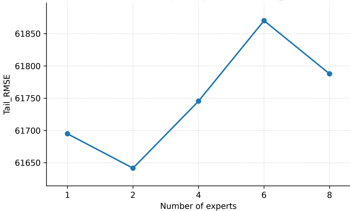
Number of Experts | Geant | PredLen=15 | Tail_RMSE
