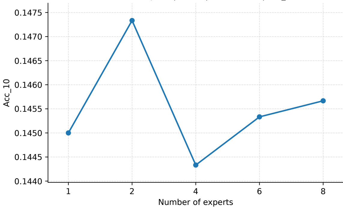
Number of Experts | Geant | PredLen=20 | Acc_10
