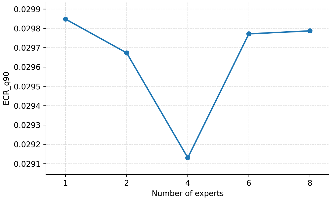
Number of Experts | Geant | PredLen=20 | ECR_q90
