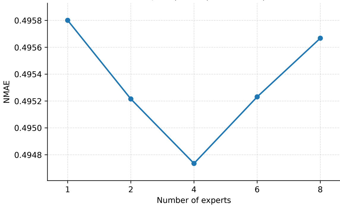
Number of Experts | Geant | PredLen=20 | NMAE
