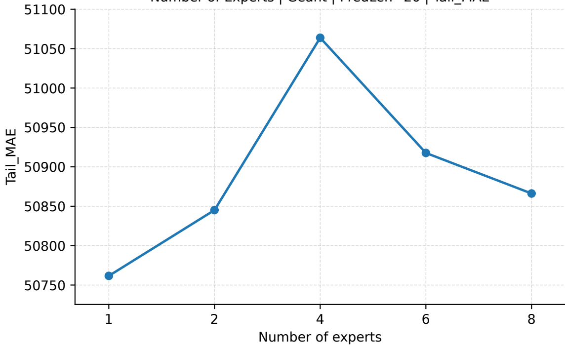
Number of Experts | Geant | PredLen=20 | Tail_MAE
