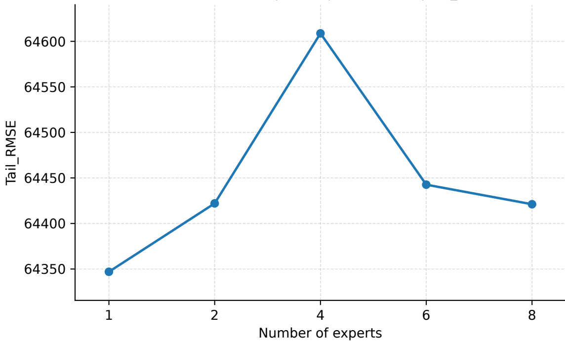
Number of Experts | Geant | PredLen=20 | Tail_RMSE
