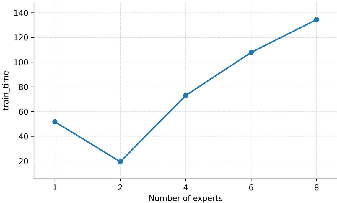
Number of Experts | Geant | PredLen=20 | train_time
