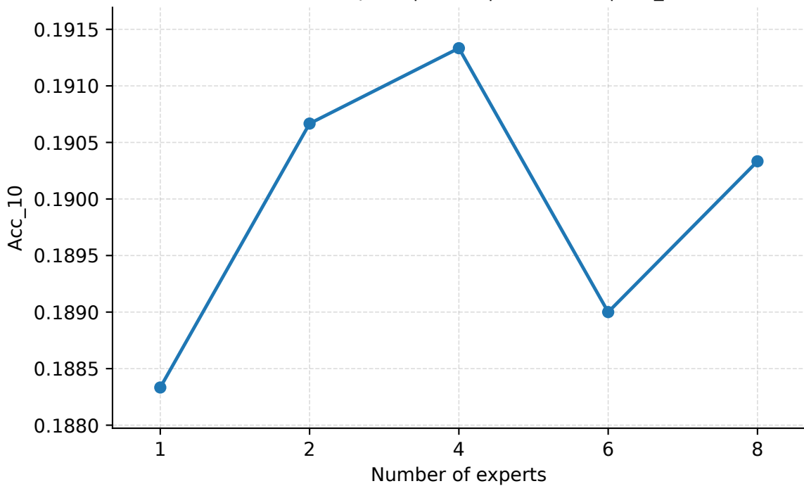
Number of Experts | Geant | PredLen=5 | Acc_10
