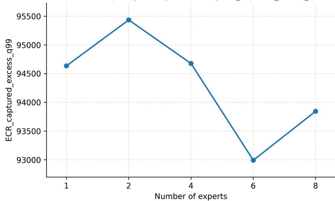
Number of Experts | Geant | PredLen=5 | ECR_captured_excess_q99
