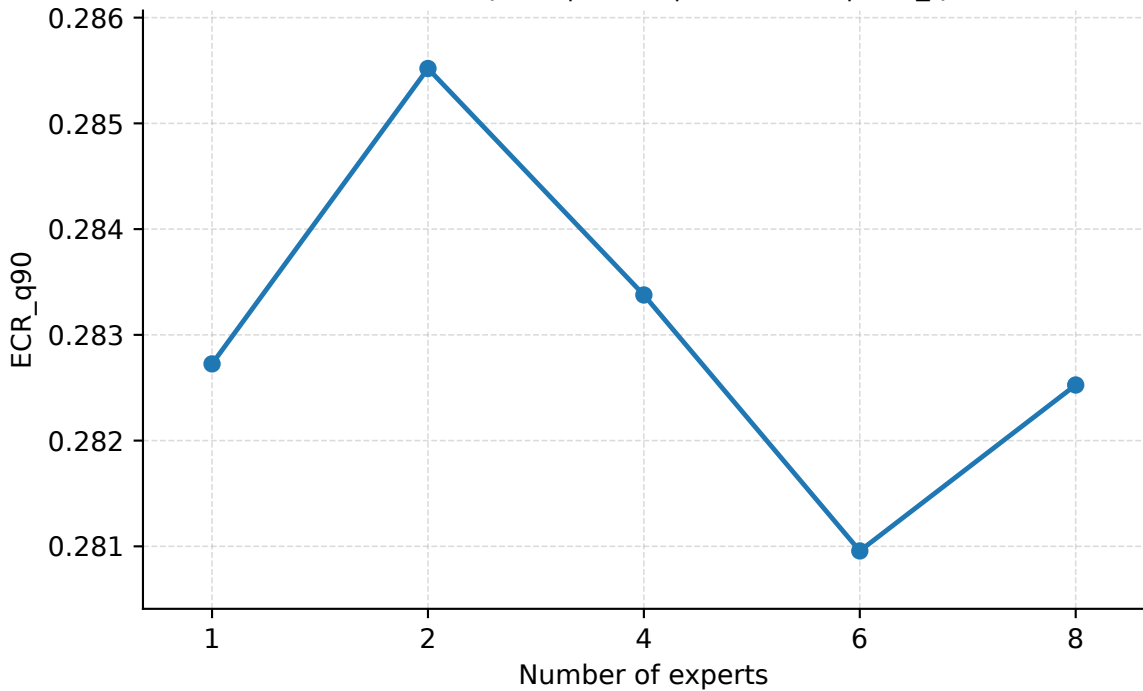
Number of Experts | Geant | PredLen=5 | ECR_q90
