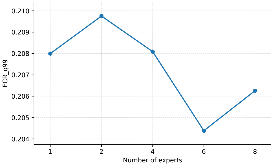
Number of Experts | Geant | PredLen=5 | ECR_q99
