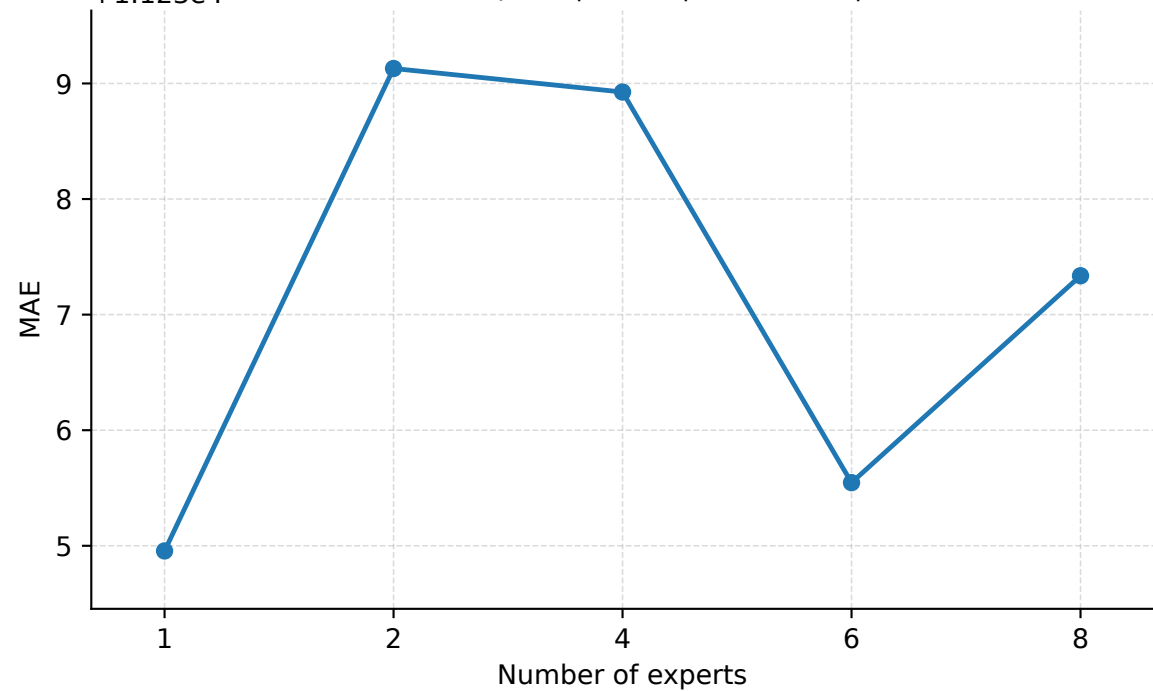
Number of Experts | Geant | PredLen=5 | MAE
