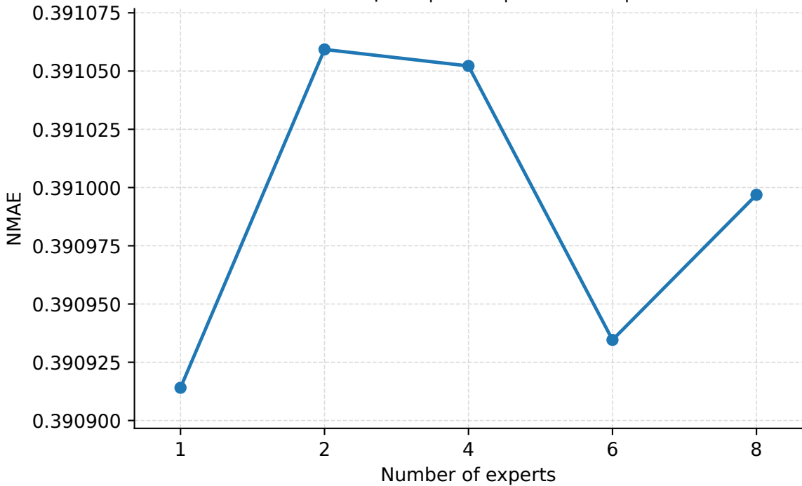
Number of Experts | Geant | PredLen=5 | NMAE
