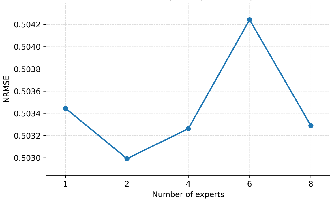
Number of Experts | Geant | PredLen=5 | NRMSE
