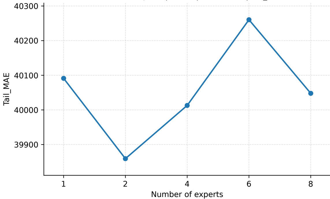
Number of Experts | Geant | PredLen=5 | Tail_MAE
