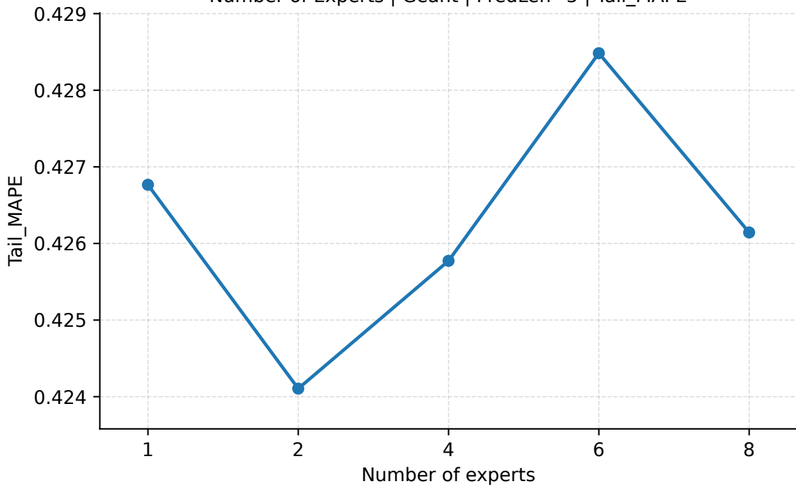
Number of Experts | Geant | PredLen=5 | Tail_MAPE
