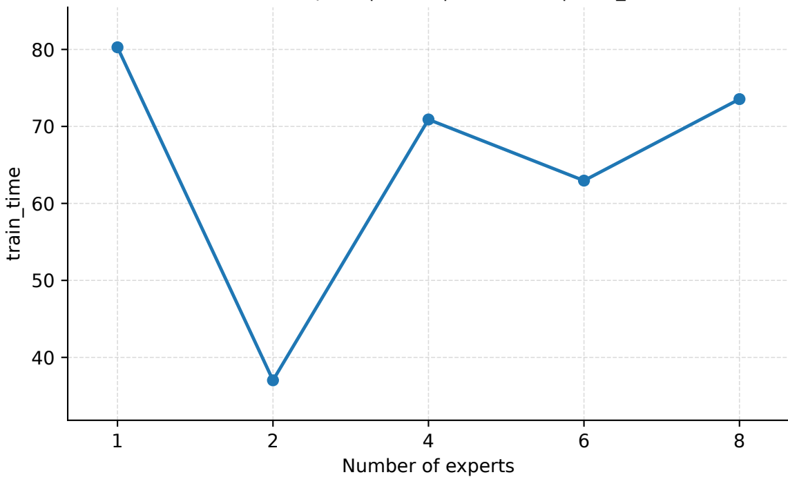
Number of Experts | Geant | PredLen=5 | train_time
