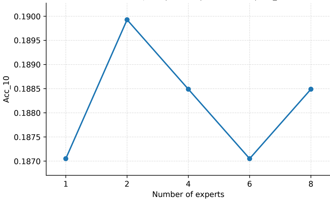
Number of Experts | Seattle | PredLen=10 | Acc_10
