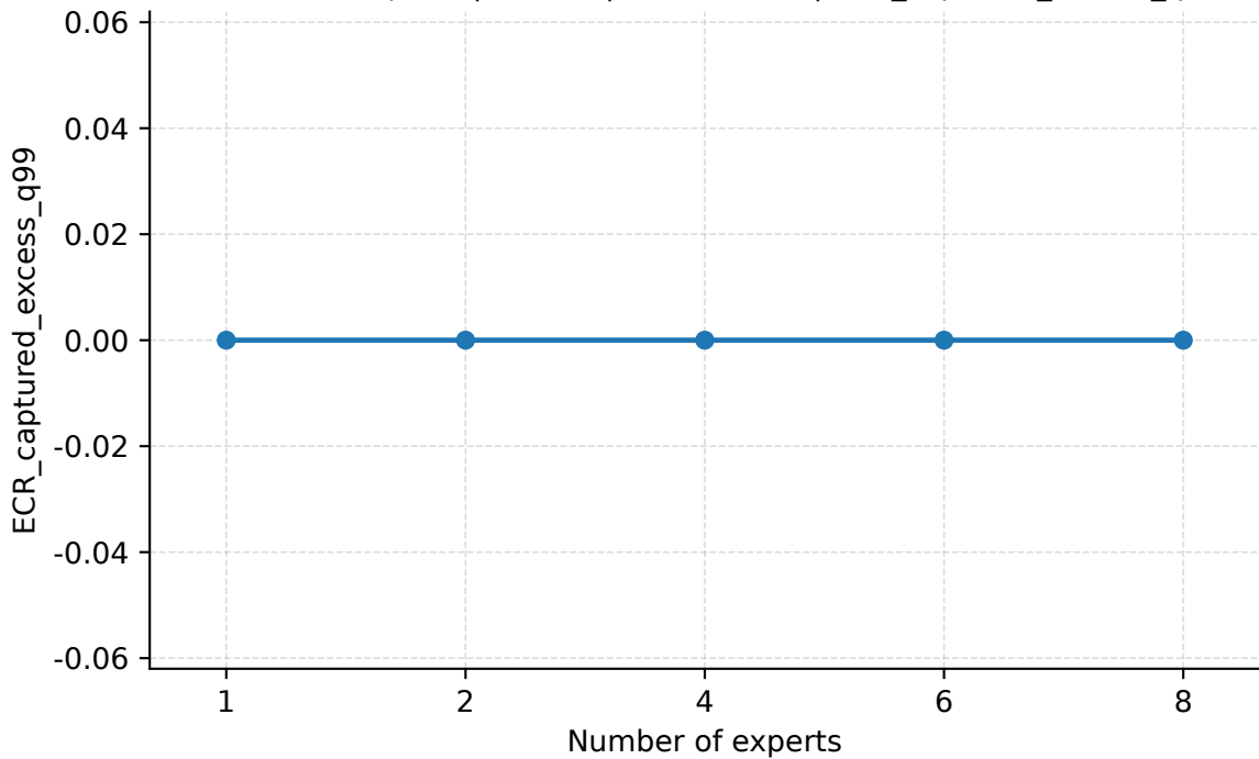
Number of Experts | Seattle | PredLen=10 | ECR_captured_excess_q99
