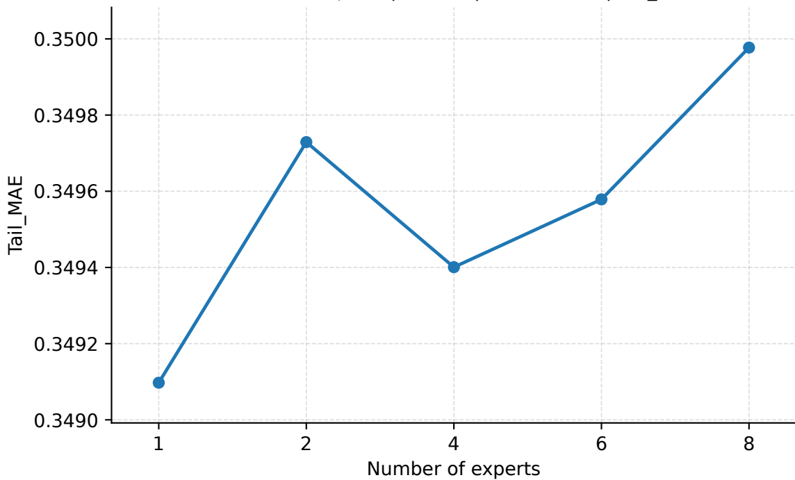
Number of Experts | Seattle | PredLen=10 | Tail_MAE
