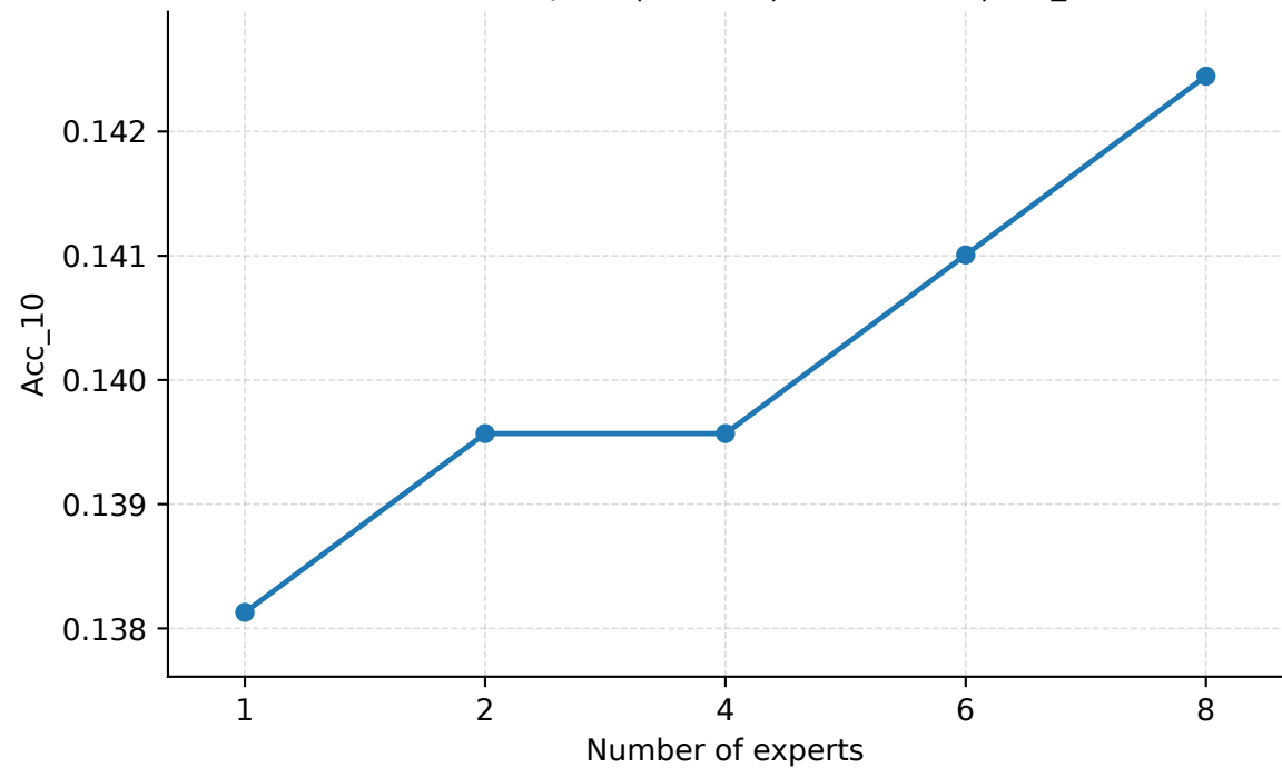
Number of Experts | Seattle | PredLen=15 | Acc_10
