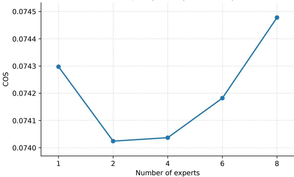
Number of Experts | Seattle | PredLen=15 | COS
