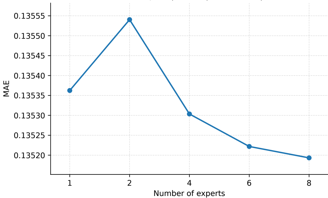
Number of Experts | Seattle | PredLen=15 | MAE
