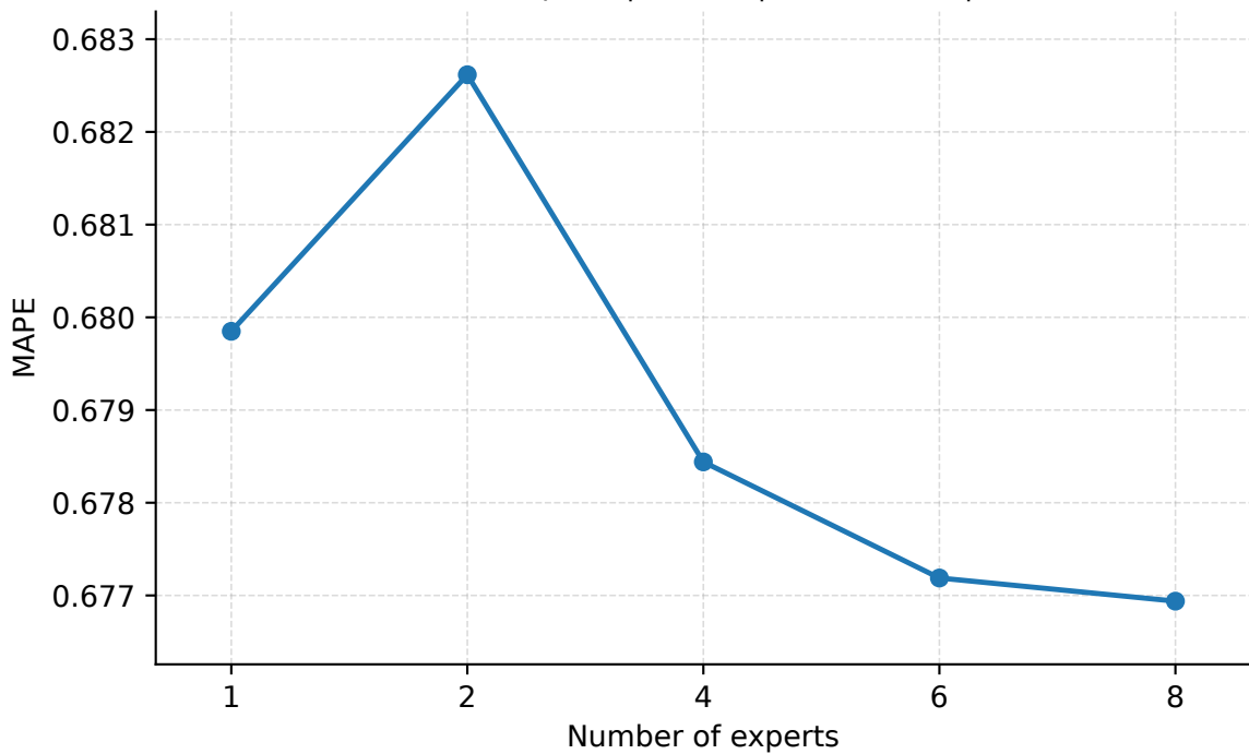
Number of Experts | Seattle | PredLen=15 | MAPE
