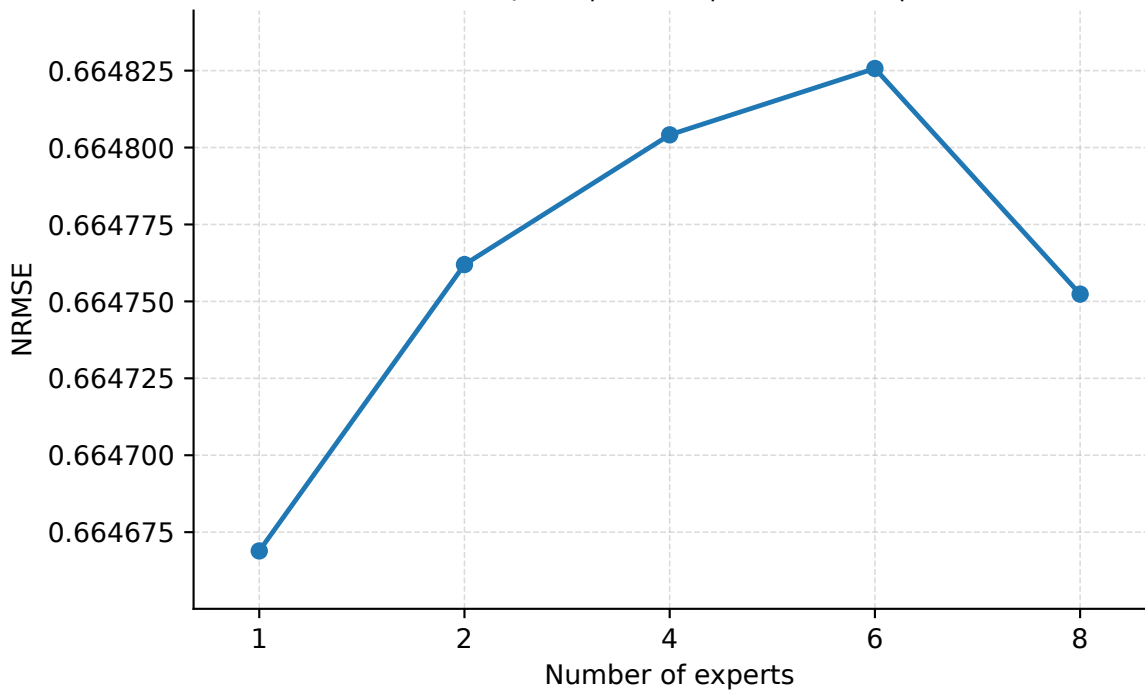
Number of Experts | Seattle | PredLen=15 | NRMSE
