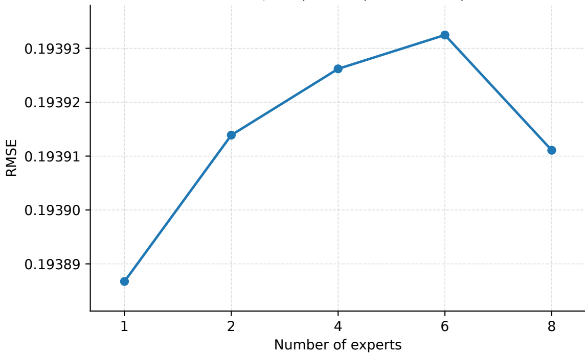
Number of Experts | Seattle | PredLen=15 | RMSE
