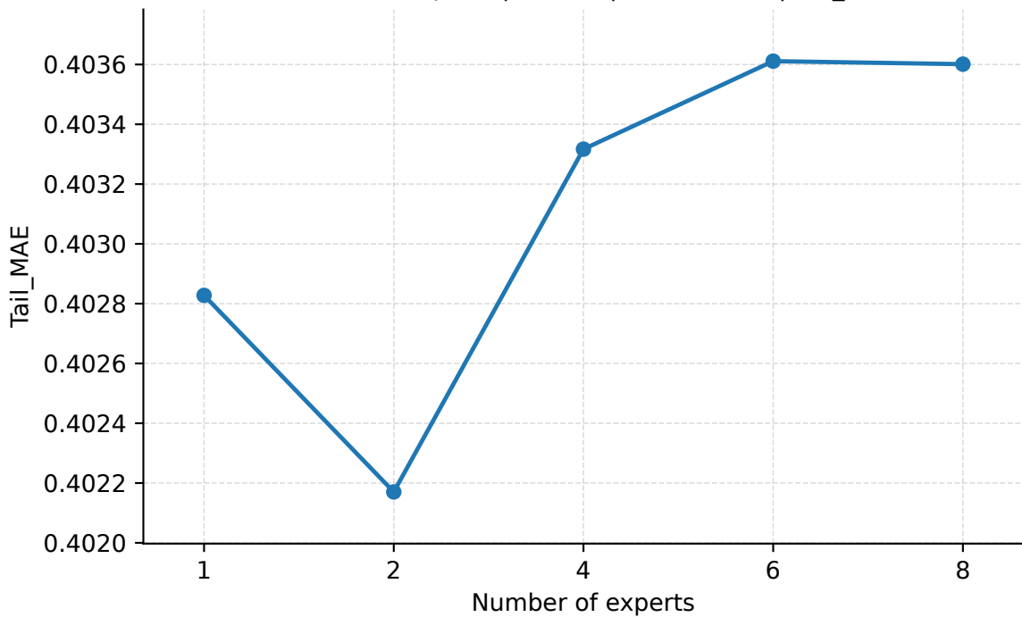
Number of Experts | Seattle | PredLen=15 | Tail_MAE
