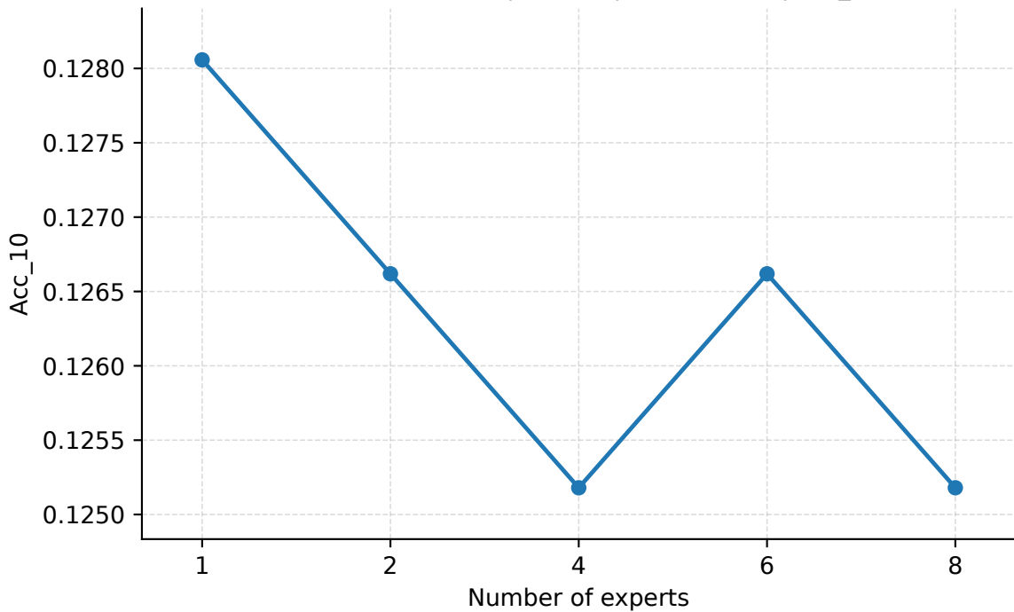
Number of Experts | Seattle | PredLen=20 | Acc_10
