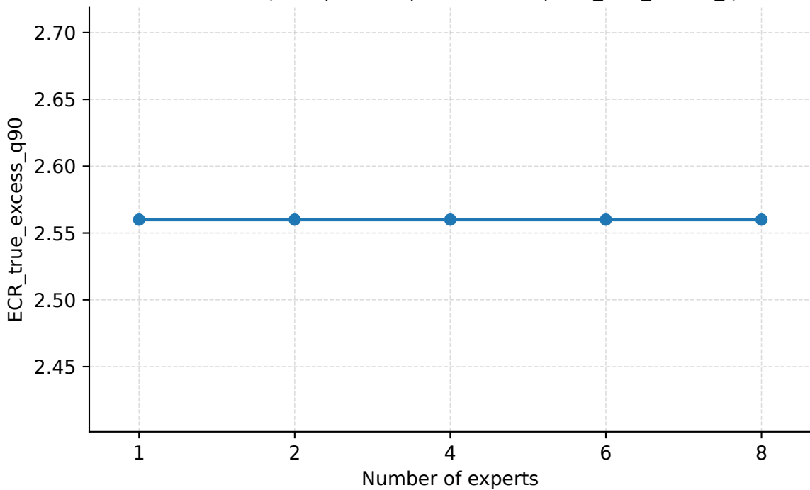
Number of Experts | Seattle | PredLen=20 | ECR_true_excess_q90
