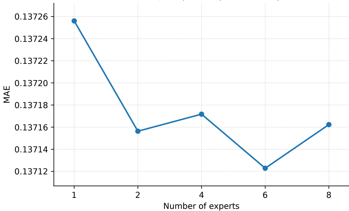
Number of Experts | Seattle | PredLen=20 | MAE
