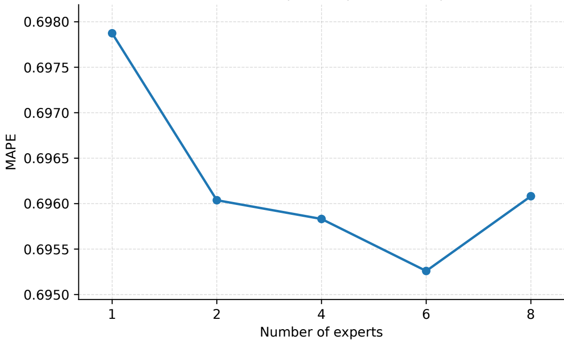
Number of Experts | Seattle | PredLen=20 | MAPE
