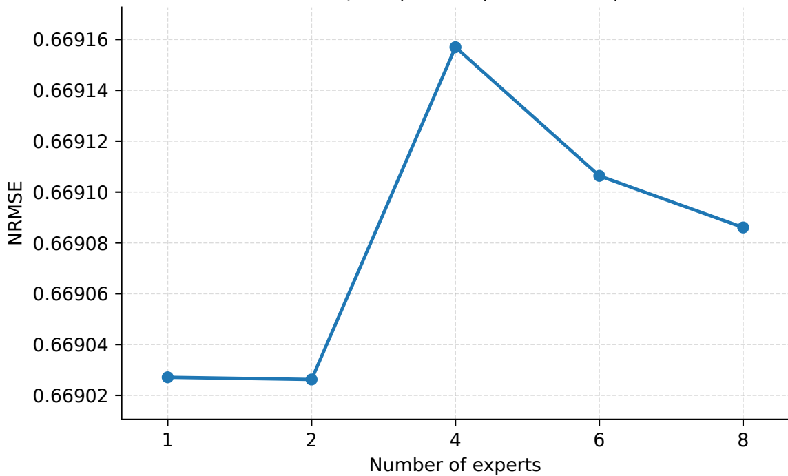
Number of Experts | Seattle | PredLen=20 | NRMSE
