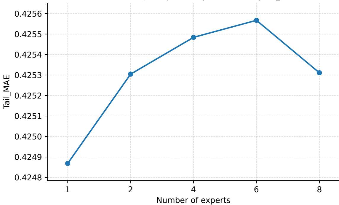
Number of Experts | Seattle | PredLen=20 | Tail_MAE
