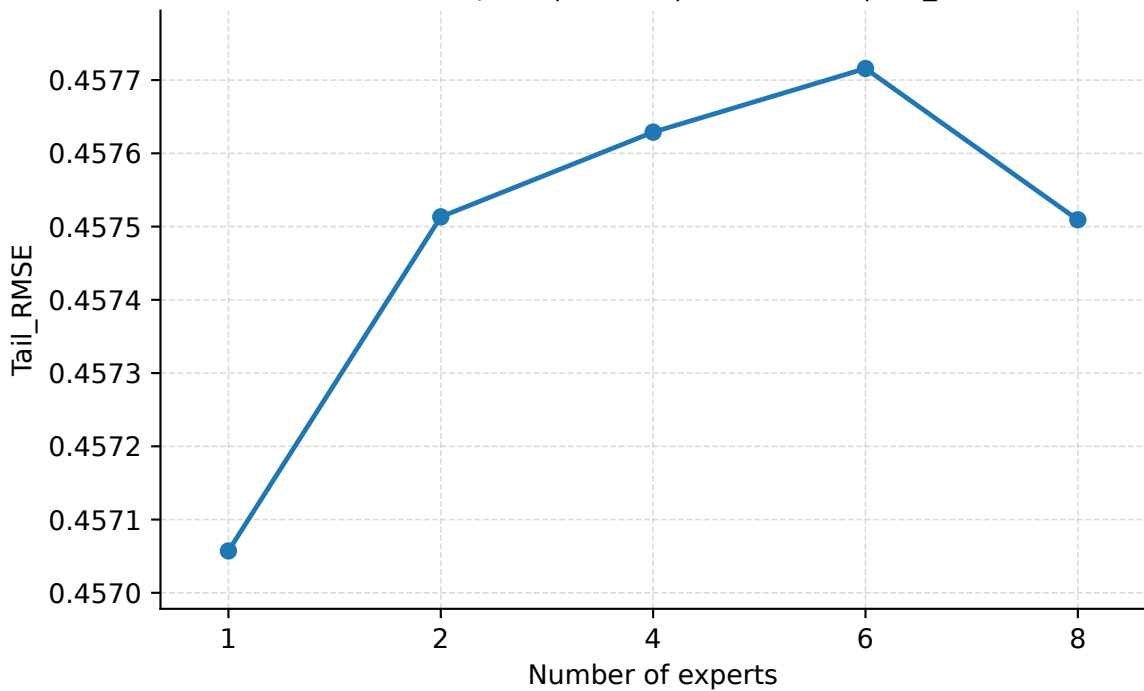
Number of Experts | Seattle | PredLen=20 | Tail_RMSE
