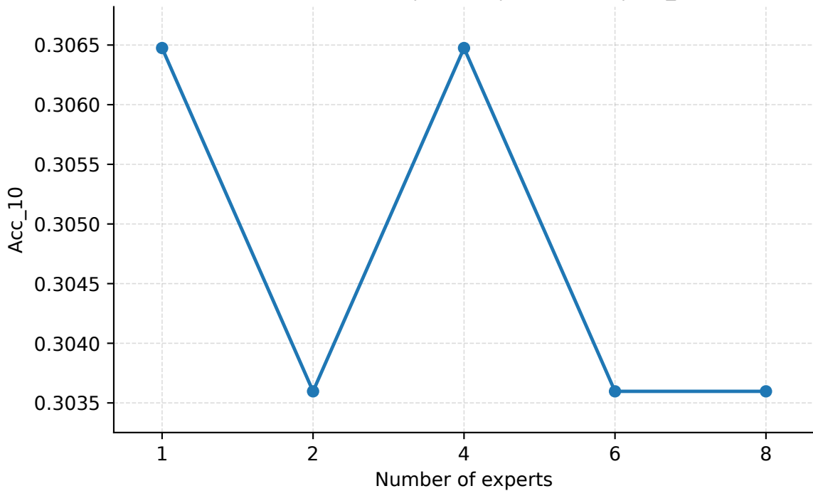
Number of Experts | Seattle | PredLen=5 | Acc_10
